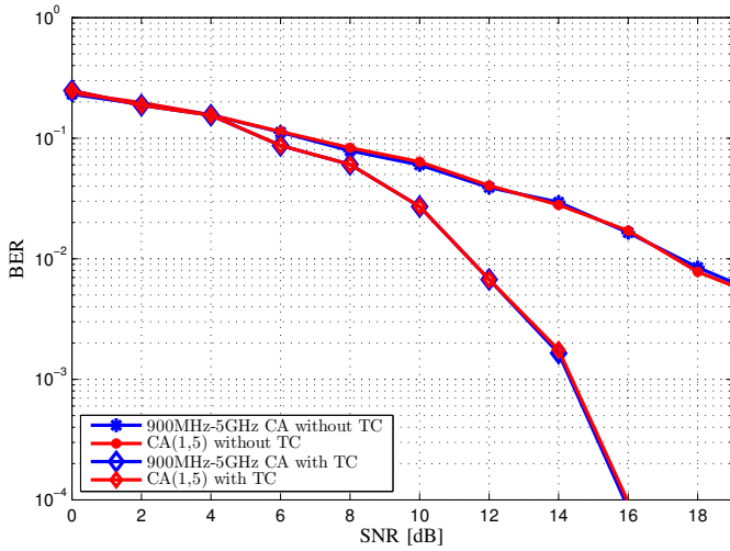
Fig. 6. Performance of two inter-band CA scenarios over dispersed bands; i) licensed CA(1,5) and ii) unlicensed 900 MHz - 5 GHz, with or without Turbo Coding (TC) and total bandwidth in both cases equal to 20 MHz.
